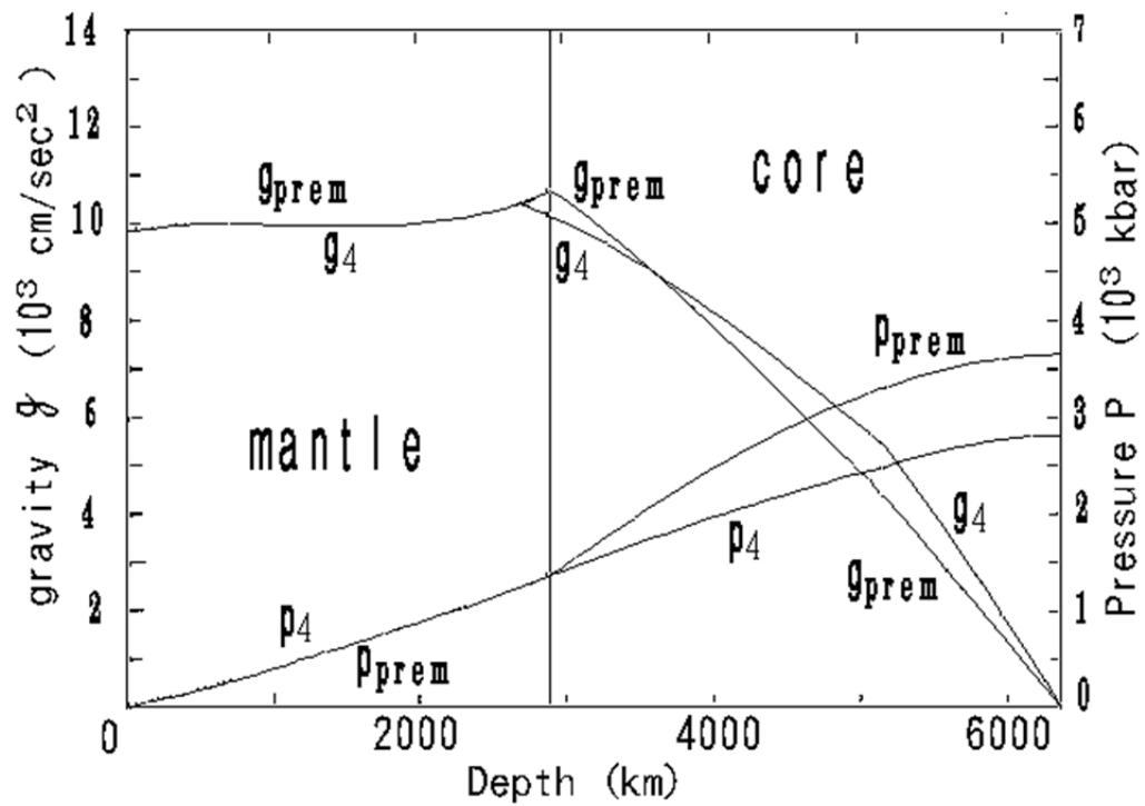
Figure 5. The gravity g and the pressure P of the new earth model and the PREM.
