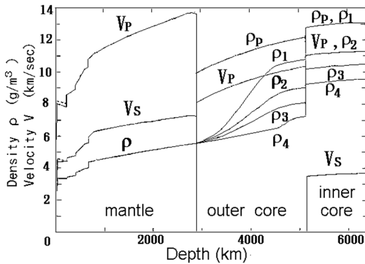
Figure 4. The density \rho of the new Earth models 1, 2, 3 and 4 compared with the PREM.
