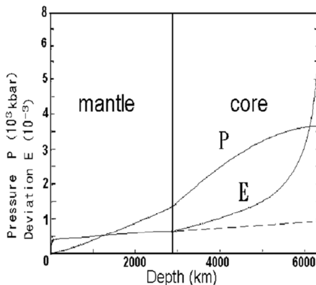
Figure 3. The pressure P of the PREM and the deviation E of the calculated pressure of simplified method from the value of P.
