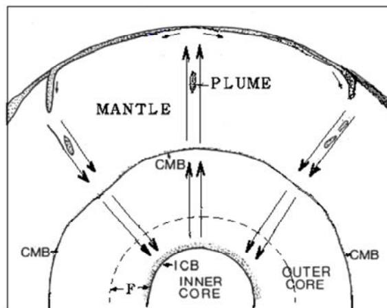
Figure 1. This is a schematic diagram of the great convection cell. A circulation of magma and solid or molten rock migrates up to the crust and down to the F zone of the outer core and causes topography of the core.
