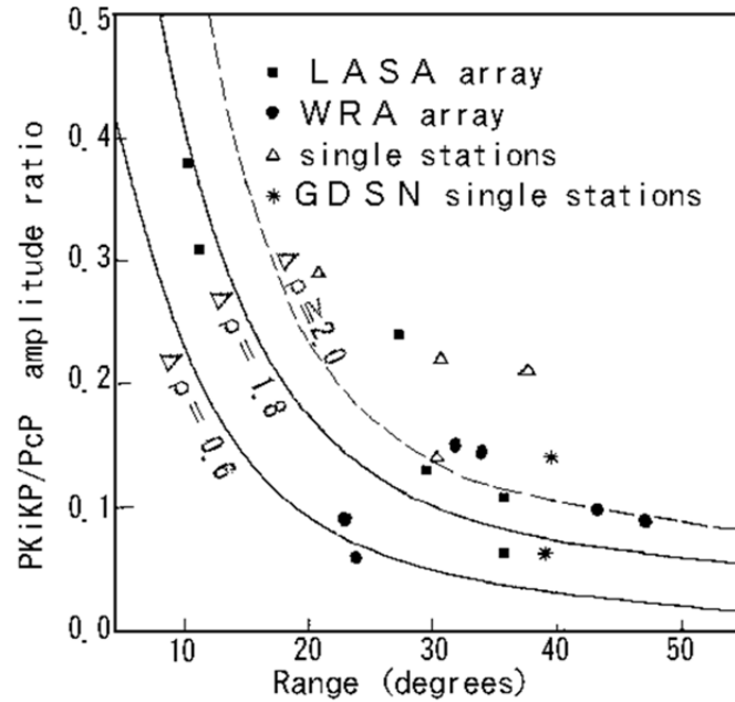
Figure 2. Observed PKiKP/PcP amplitude ratios plotted as a function of range. Solid squares indicate LASA array data [Engdahl et al. , 1970, 1974]; open triangles are single-station data [Buchbinder et al. , 1973]; solid circles are Warramunga array data [Souriau & Souriau, 1989]; stars are single-station GDSN data [Shearer & Masters, 1990]. The lower curve shows the theoretical amplitude ratio for PREM ( \rho = 0.6 \text{ g/cm}^3 ). The middle curve shows the result for a higher density contrast ( \rho = 1.8 \text{ g/cm}^3 ). The upper dashed curve shows a more reasonable curve of mean value among all the scattered points for a favorable density contrast ( \rho \geq 2.0 \text{ g/cm}^3 ).
