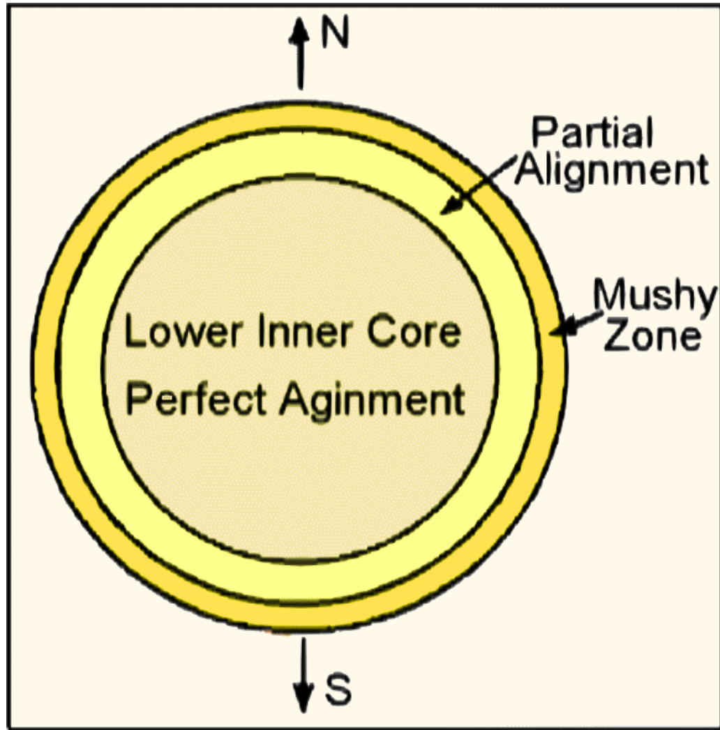
A schematic figure of inner core structure
