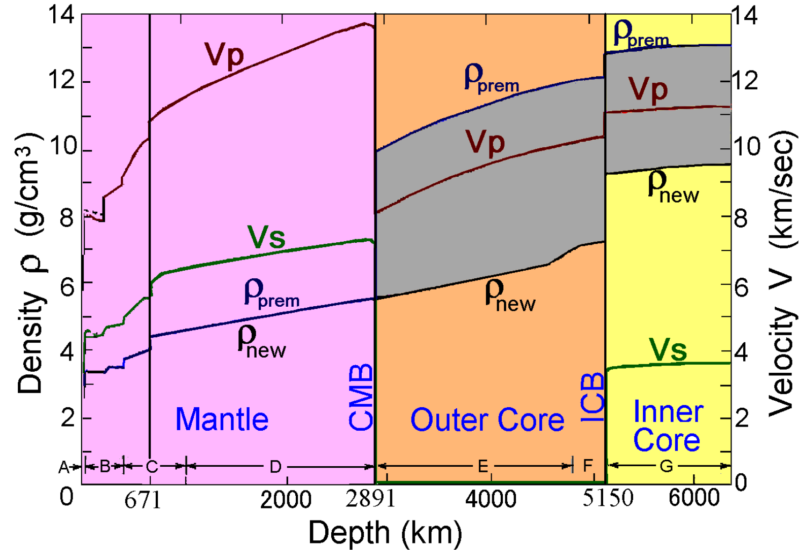
Data of PREM and the new Earth model
