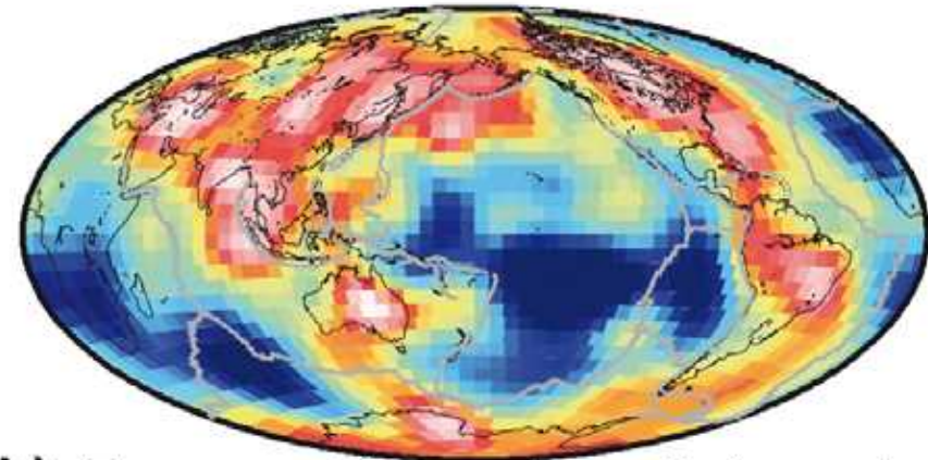
(b) Tomographic-geodynamic inversion
