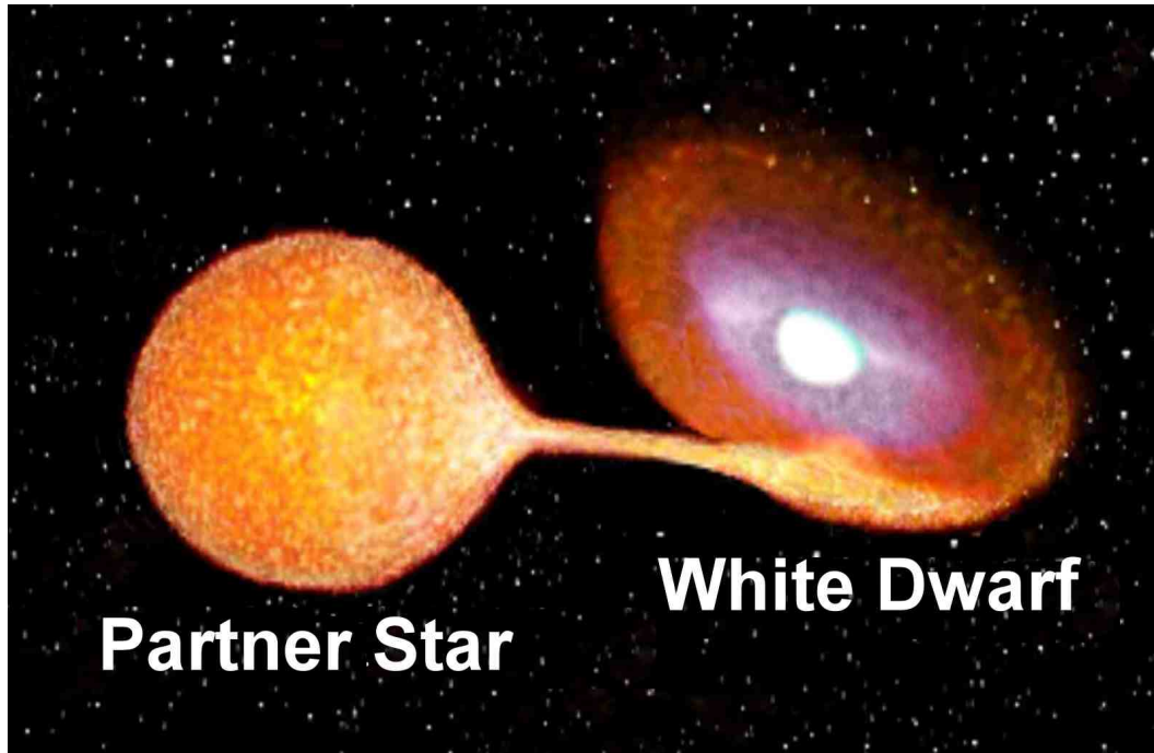
Type 1a supernovae of double star system
