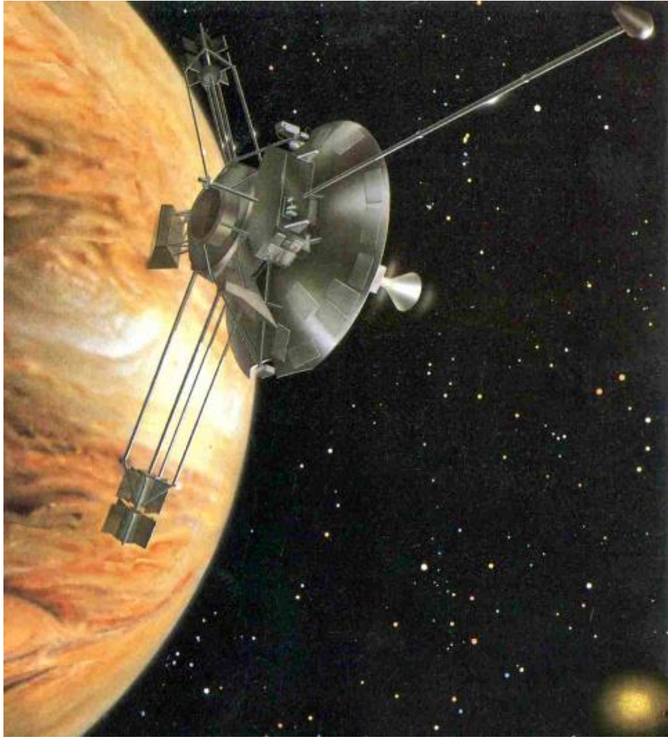
Space probe pioneer 10 arrived near Saturn
