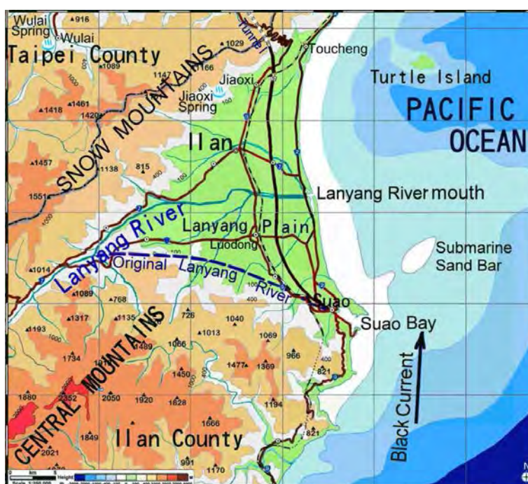
The Map of original Lanyang River.
