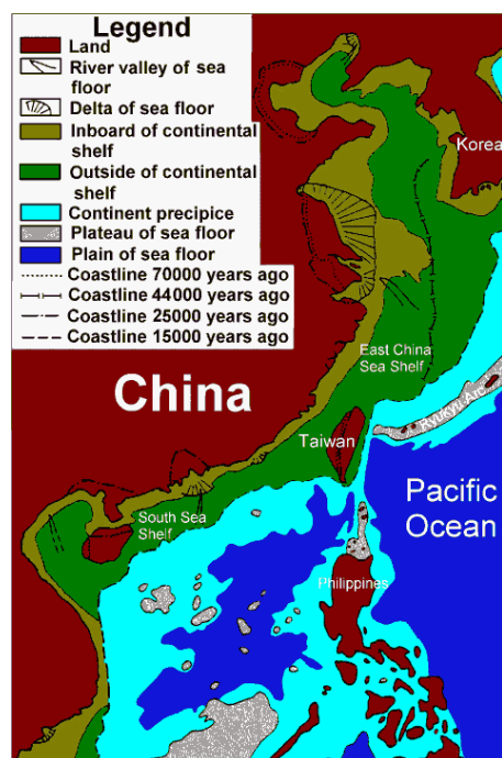
Topographic map of 4th glacial age.
