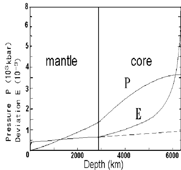
Figure 3. The pressure P of the PREM and the deviation E of the calculated pressure of simplified method from the value of P .
