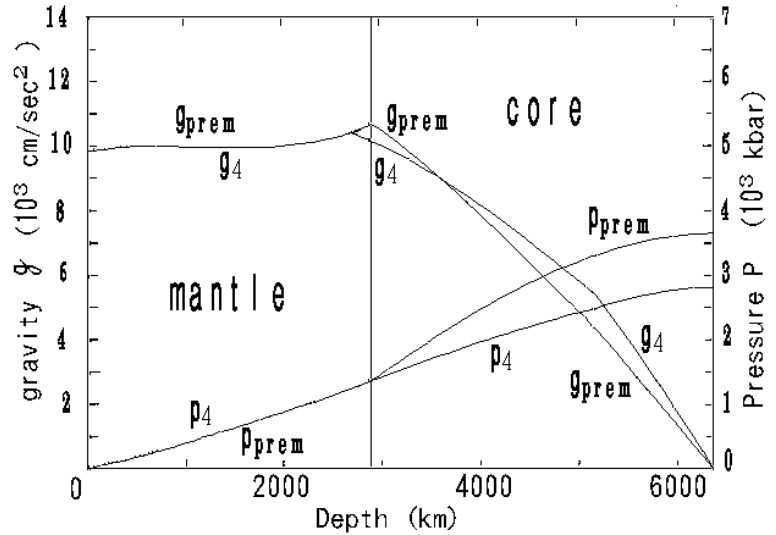
Figure 5. The gravity and the pressure P of the new earth model and the PREM.
