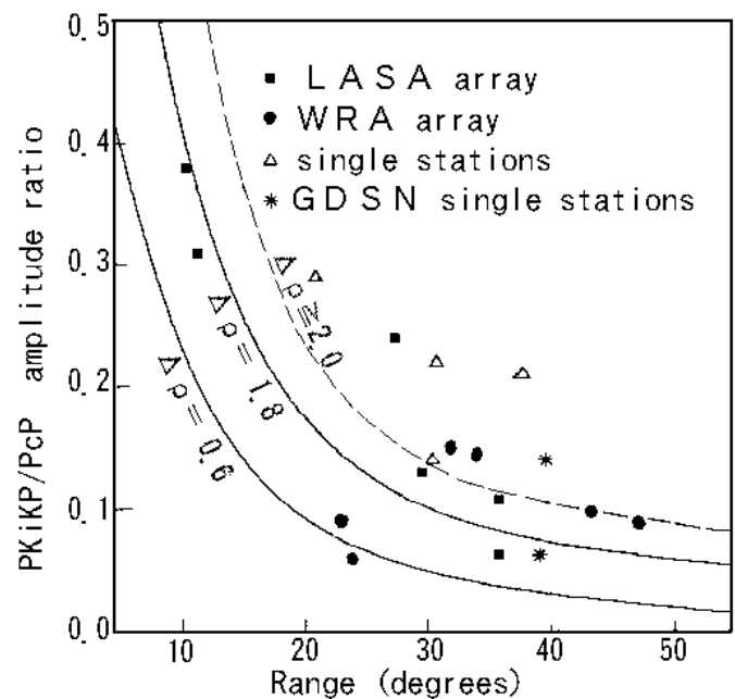
Figure 2. Observed PKiKP/PcP amplitude ratios plotted as a function of range. Solid squares indicate LASA array data (Engdahl et al., 1970, 1974); open triangles are single-station data (Buchbinder et al., 1973); solid circles are Warramunga array data (Souriau & Souriau, 1989); stars are single-station GDSN data (Shearer & Masters, 1990). The lower curve shows the theoretical amplitude ratio for PREM ( \rho = 0.6 \text{ g/cm}^3 ). The middle curve shows the result for a higher density contrast ( \rho = 1.8 \text{ g/cm}^3 ). The upper dashed curve shows a more reasonable curve of mean value among all the scattered points for a favorable density contrast ( \rho \geq 2.0 \text{ g/cm}^3 ).
