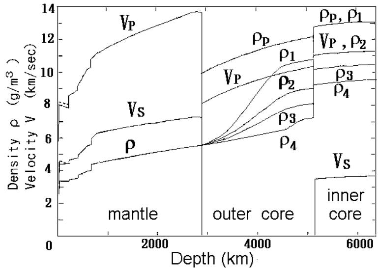
Figure 4. The density of the new Earth models 1, 2, 3 and 4
