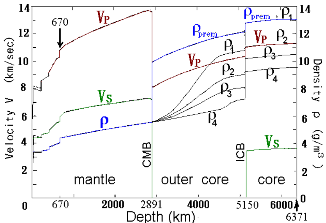
Figure 6. The density \rho of the new Earth models 1, 2, 3 and 4 compared with the PREM.
