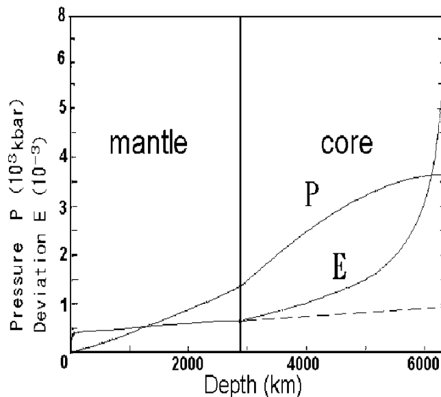
Figure 5. The pressure P of the PREM and the deviation E of the calculated pressure of simplified method from the value of P.
