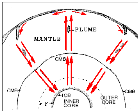
Figure 3. This is a schematic diagram of the great convection cell. A circulation of magma and solid or molten rock migrates up to the crust and down to the F zone of the outer core and causes topography of the core.
