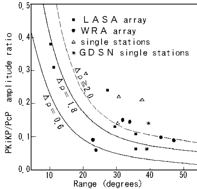
Figure 4. Observed PKiKP/PcP amplitude ratios plotted as a function of range. Solid squares indicate LASA array data [Engdahl et al. , 1970, 1974]; open triangles are single-station data [Buchbinder et al. , 1973]; solid circles are Warramunga array data [Souriau & Souriau, 1989]; stars are single-station GDSN data [Shearer & Masters, 1990]. The lower curve shows the theoretical amplitude ratio for PREM ( \rho = 0.6 \text{ g/cm}^3 ). The middle curve shows the result for a higher density contrast ( \rho = 1.8 \text{ g/cm}^3 ). The upper dashed curve shows a more reasonable curve of mean value among all the scattered points for a favorable density contrast ( \rho \geq 2.0 \text{ g/cm}^3 ).
