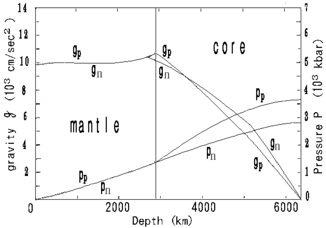
Figure 7. The distribution of gravity g and the pressure P of the PREM( p ) and the new earth model( n ).
